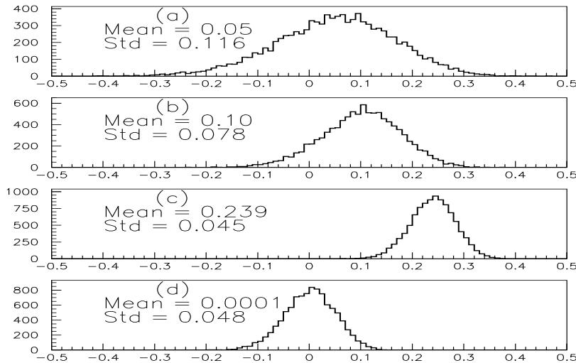
Fig. 1. Distribution of \frac{\int_0^1 \sigma^2(t)dt - \hat{\sigma}^2}{\int_0^1 \sigma^2(t)dt} , where \hat{\sigma}^2 are three different estimators of the integrated volatility: (a) estimator (11) with m = 144 ; (b) estimator (11) with m = 288 ; (c) estimator (11) with m = 720 ; (d) Fourier estimator (12). The distribution is computed with 10,000 “daily” replications.
